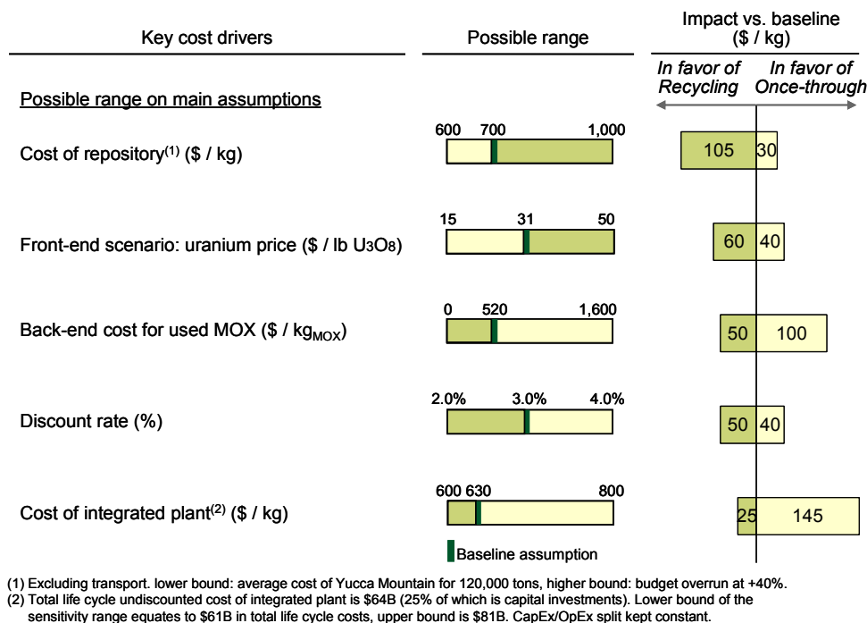
Figure 11: Summary of main sensitivities in Greenfield approach
