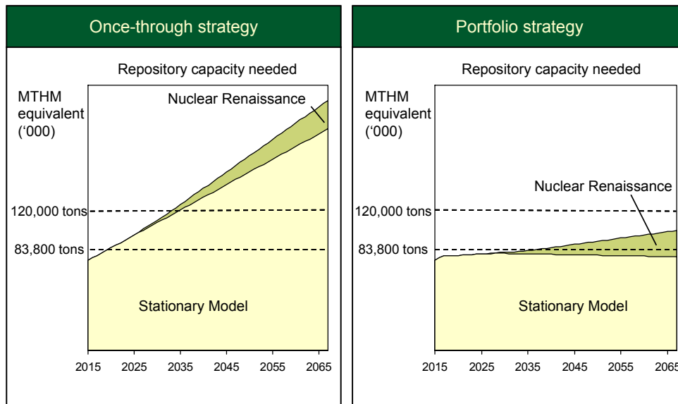
Figure 21: Impact of nuclear renaissance on repository capacity needed
