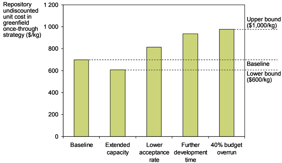
Figure 33: Sensitivity range for repository costs
