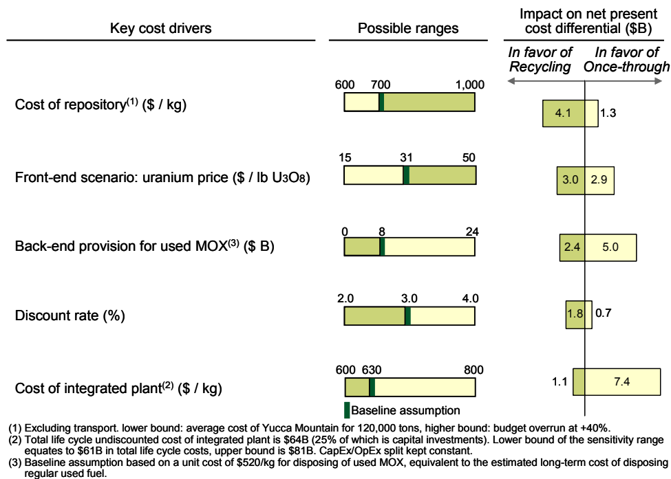
Figure 16: Summary of main sensitivities for Implementation approach
