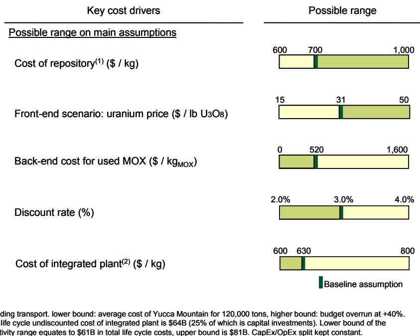
Figure 32: Summary of main sensitivities
