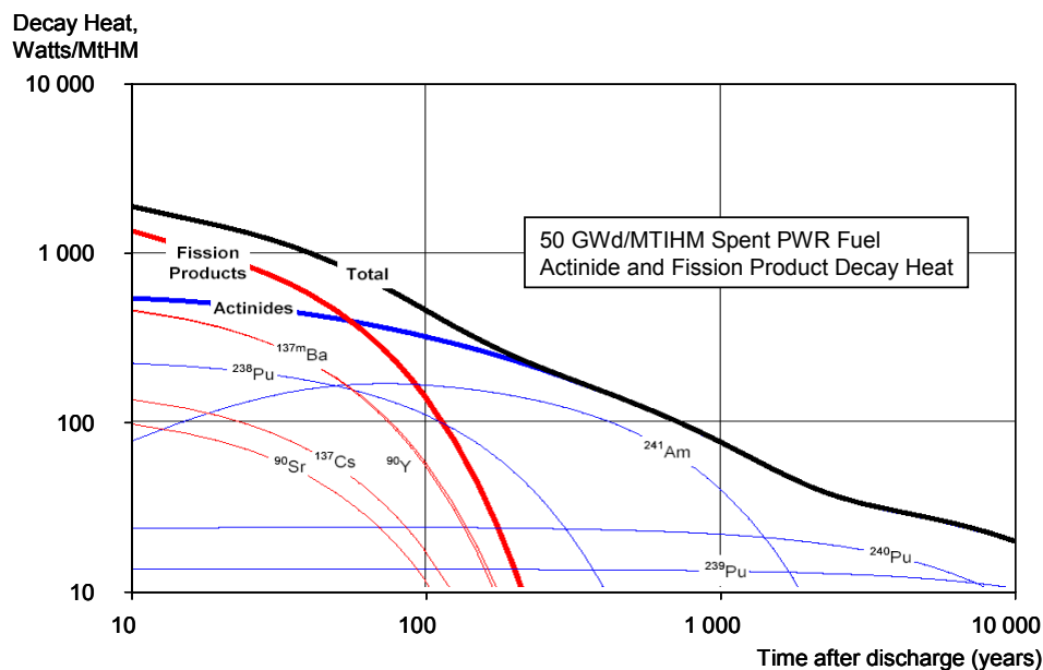
Figure 29: Contribution of each component of used fuel to the decay heat
