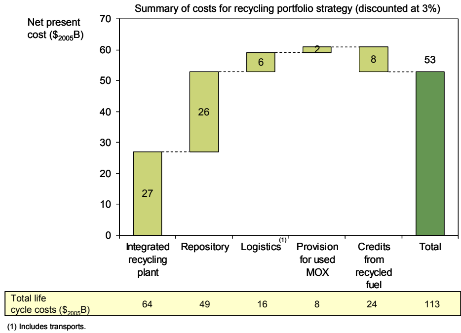
Figure 13: Cost breakdown of portfolio strategy in the Implementation approach
