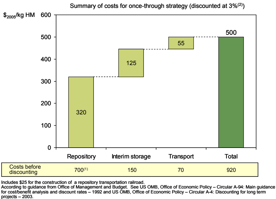
Figure 7: Cost breakdown of once-through strategy in Greenfield approach
