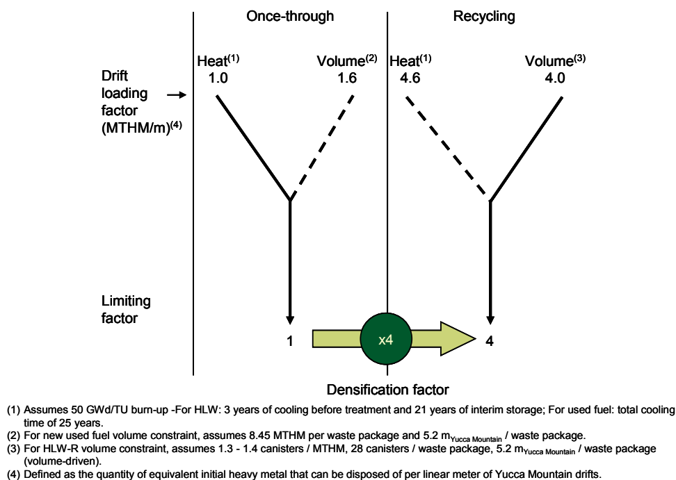
Figure 28: Densification factor calculation
