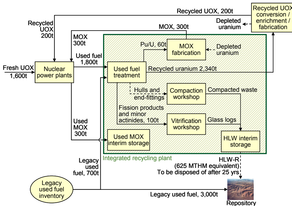
Figure 25: Annual material flows at steady state in portfolio strategy (illustrative for 2040)
