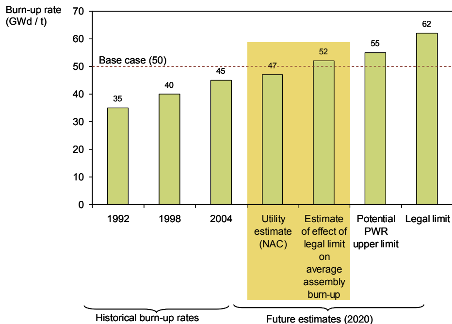
Figure 24: Burn-up rate estimates
