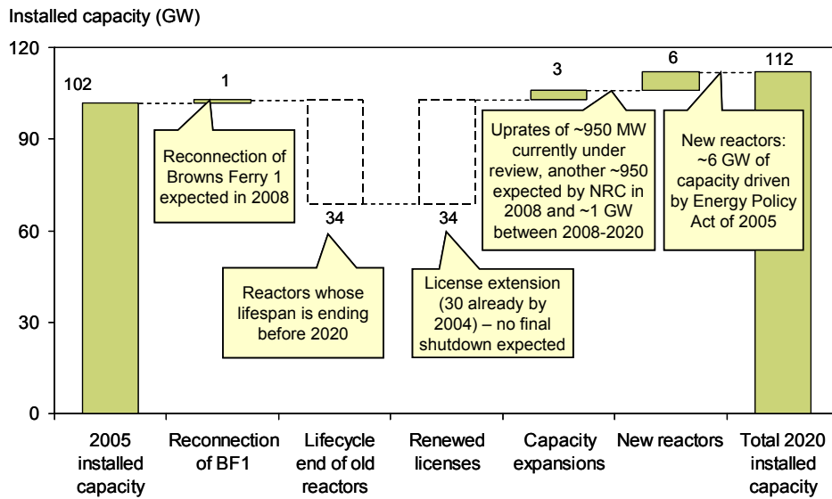
Figure 23: Expected nuclear installed capacity in 2020
