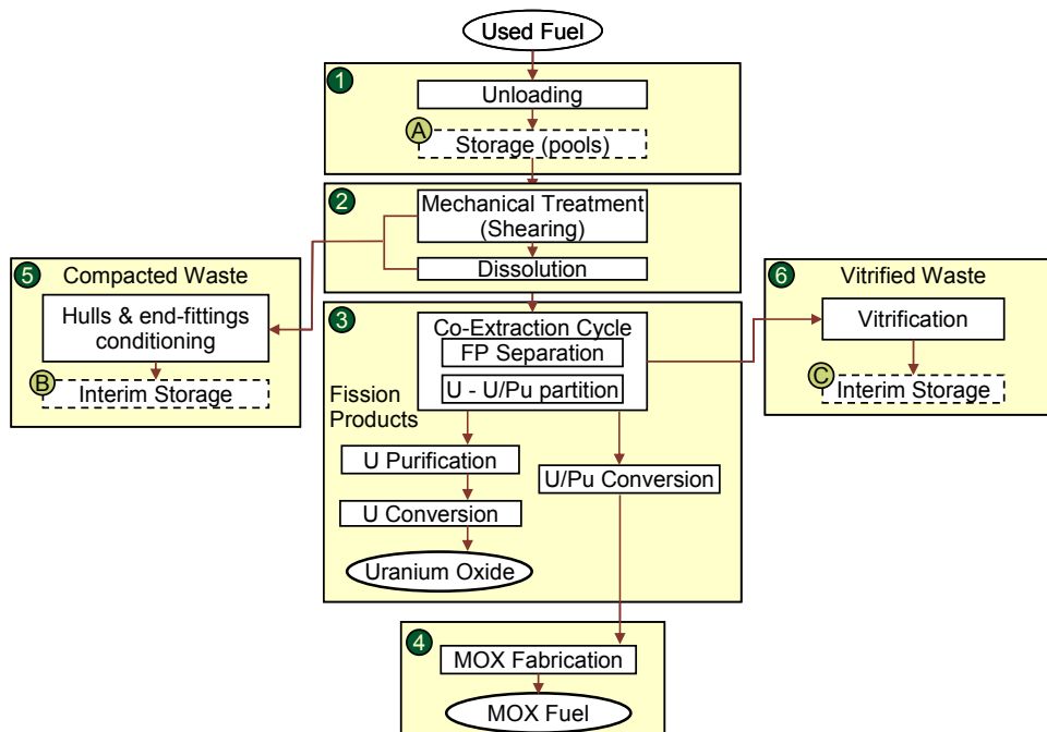
Figure 27: Schematic of the process flows within the integrated plant.
